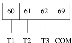
Fig 7 Communication, pulse connection
